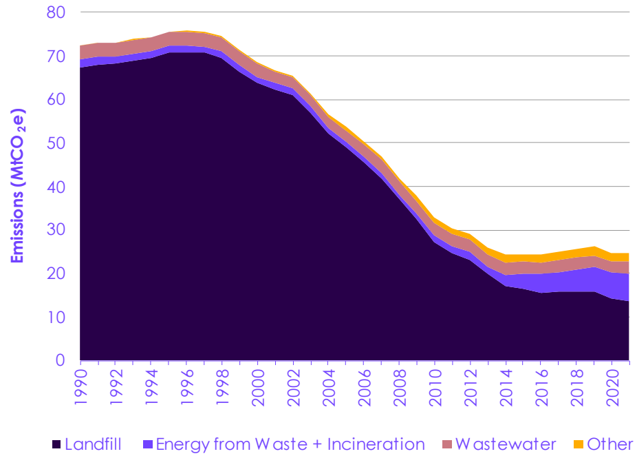
Figure 12.3 Waste emissions (1990-2021)
