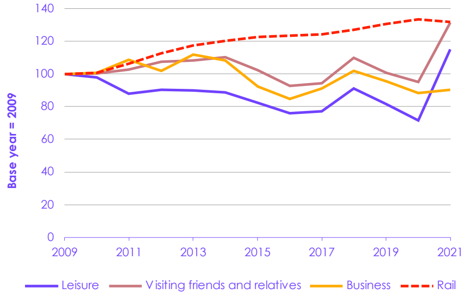
Figure 10.7 Trends in short-haul flight prices and rail
